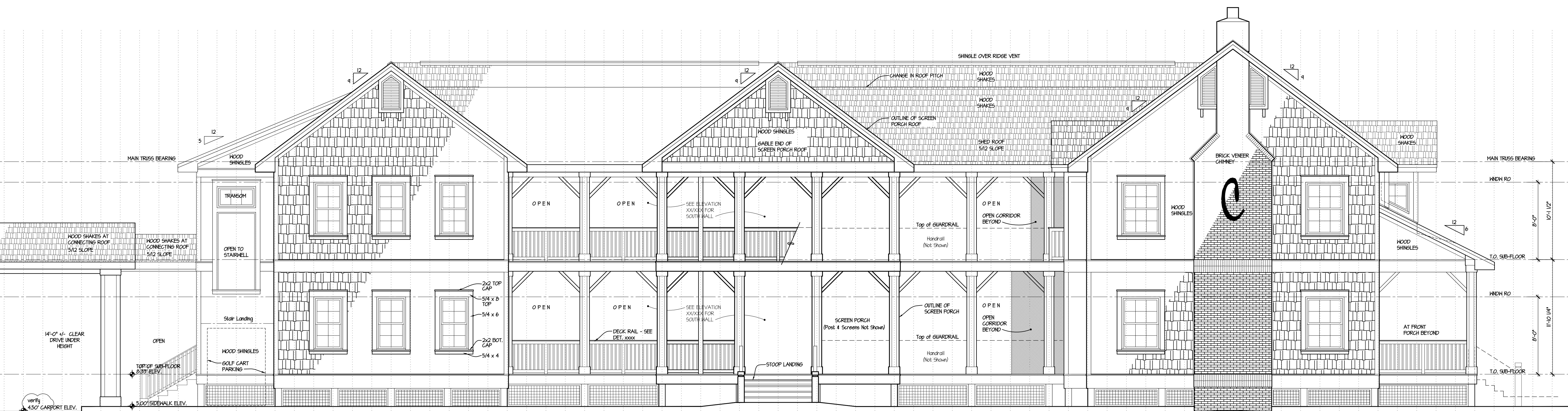
H1 PARTIAL LEFT SIDE (SOUTH) ELEVATION AT DRIVE UNDER 1/4" = 1'-0"
