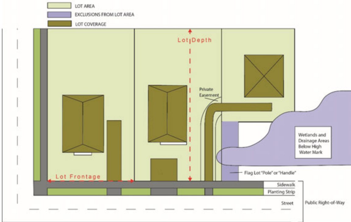
Figure 10.3.3.A.1, Lot Dimensions
