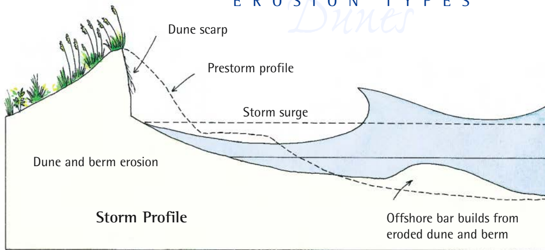
Figure D: Storm-induced erosion is caused by a single, infrequent but severe storm or hurricane.
