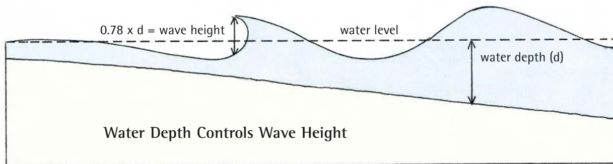
Figure A: Maximum wave height is controlled by water depth. Shallow water causes the wave to break.
