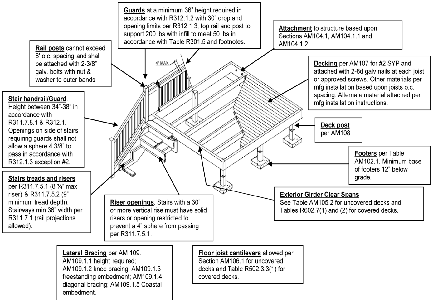
FIGURE AM111.1 DECK CONSTRUCTION
