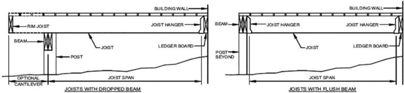
FIGURE AM106.1 TYPICAL DECK JOIST SPANS
