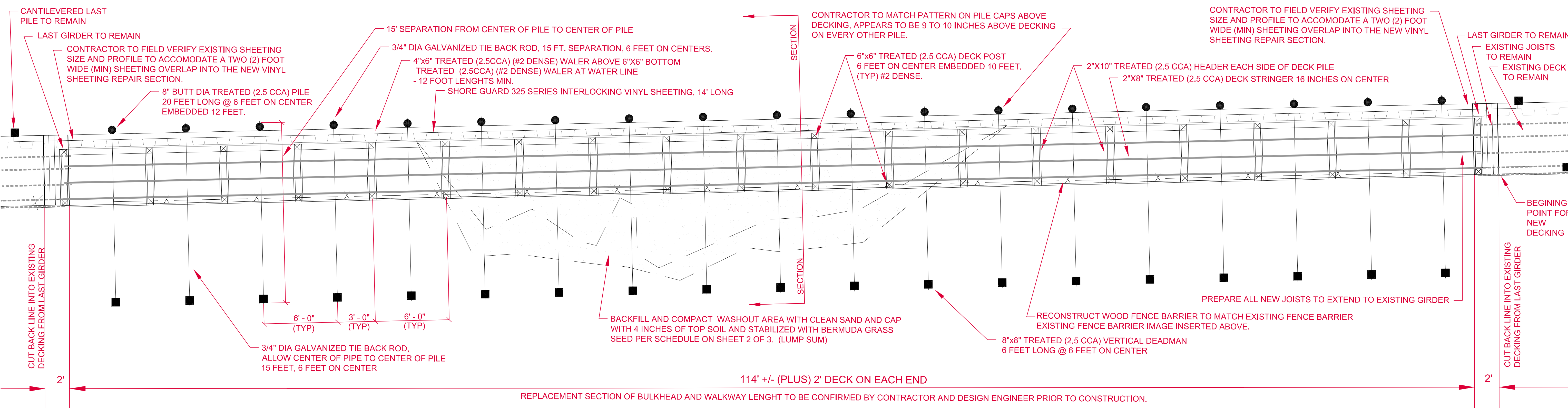
TYPICAL SECTION OF BULKHEAD & PIER REPAIR DETAIL NOT TO SCALE
