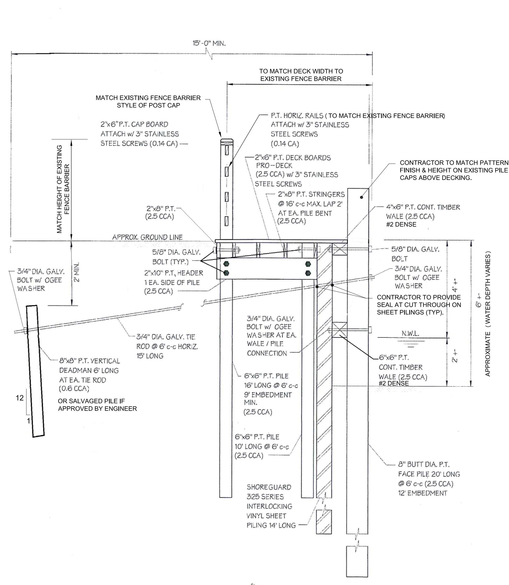
TYPICAL SECTION OF BULKHEAD & PIER REPAIR DETAIL NOT TO SCALE
