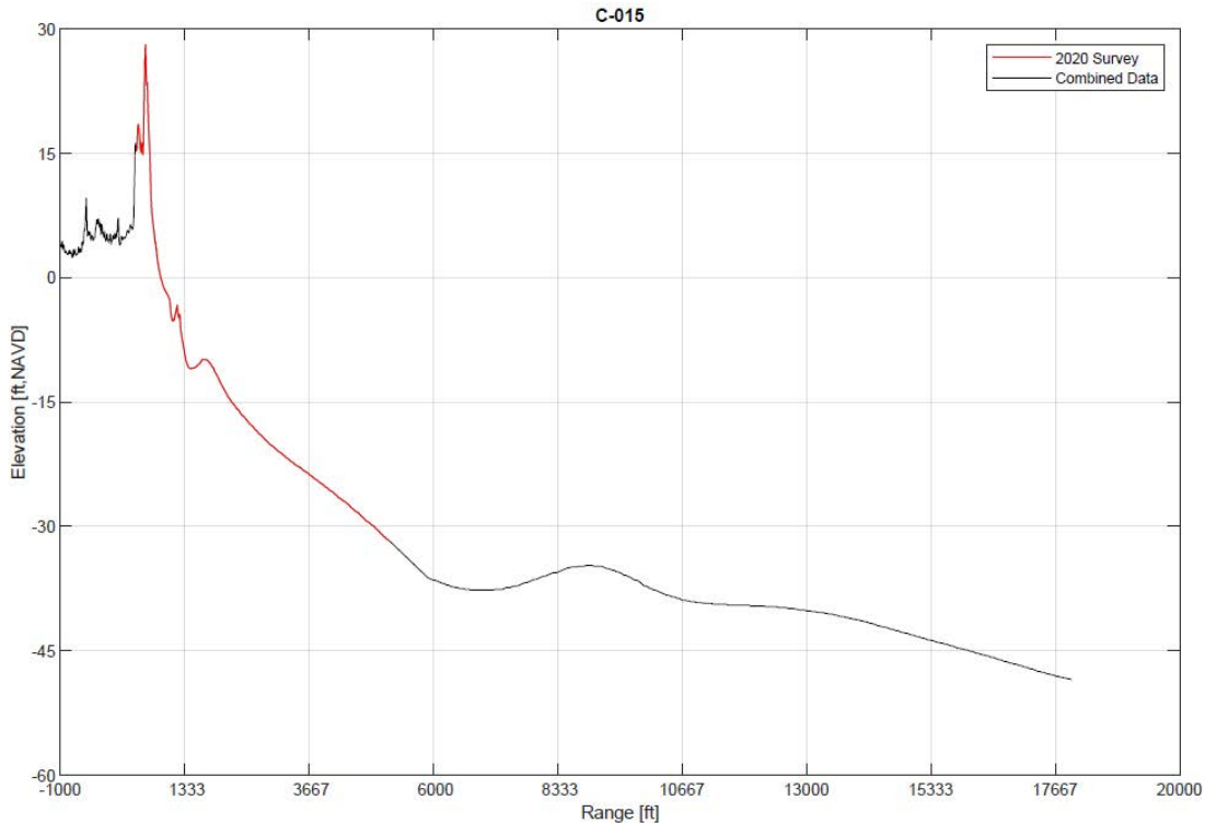
Figure 21. Typical SBEACH Profile
